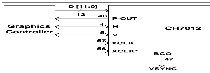
Figure 4: Master Clock Mode
