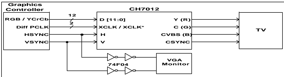
Figure 3: Sync Buffers
