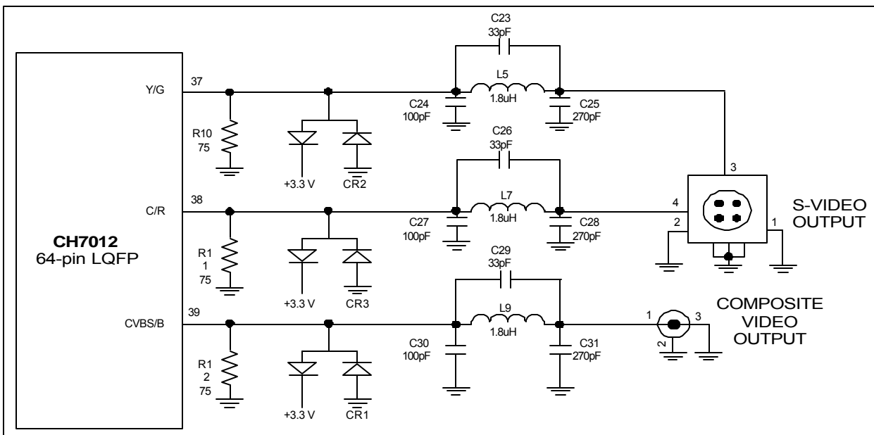
Figure 10: S-Video and Composite Video Outputs
