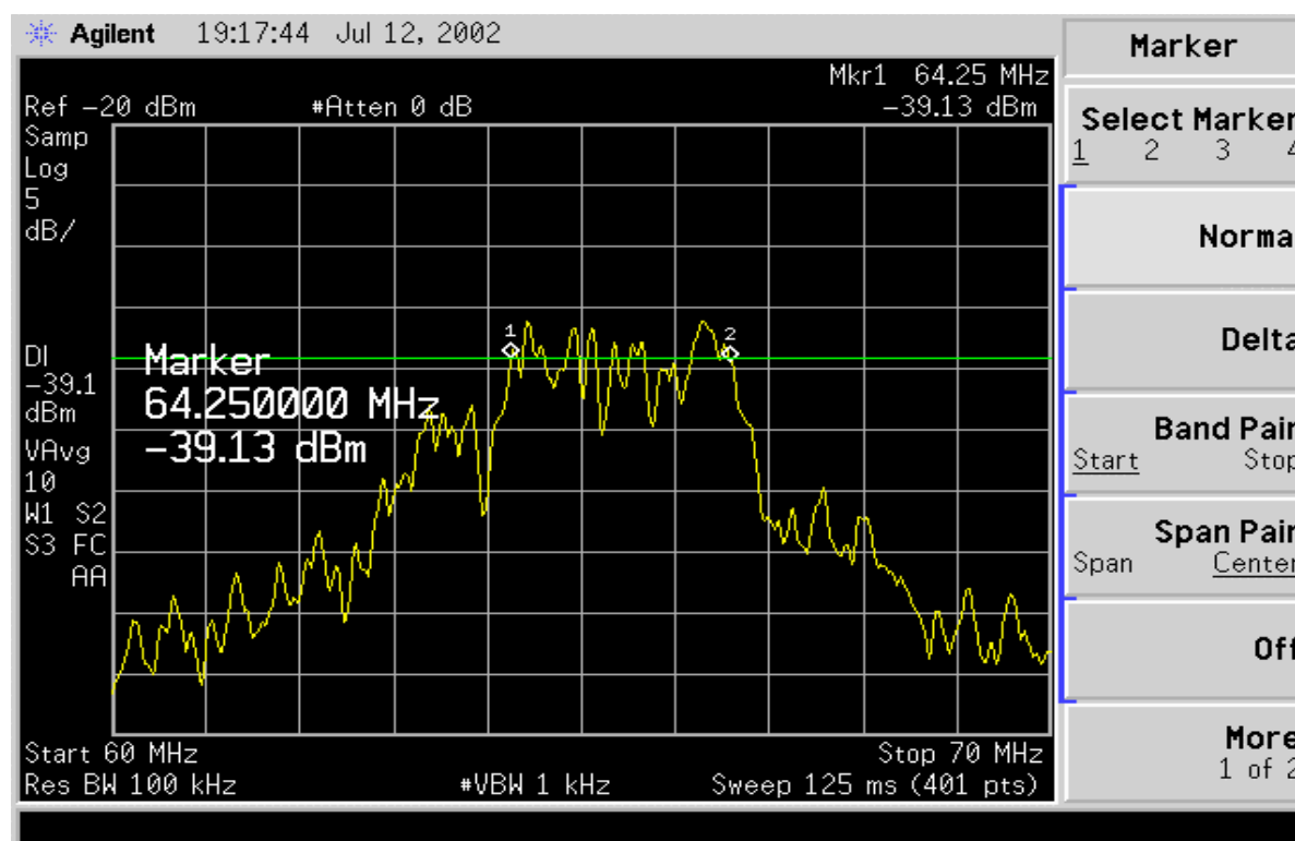
Figure 4: EMI emission reduction operation 2.5% clock spreading
