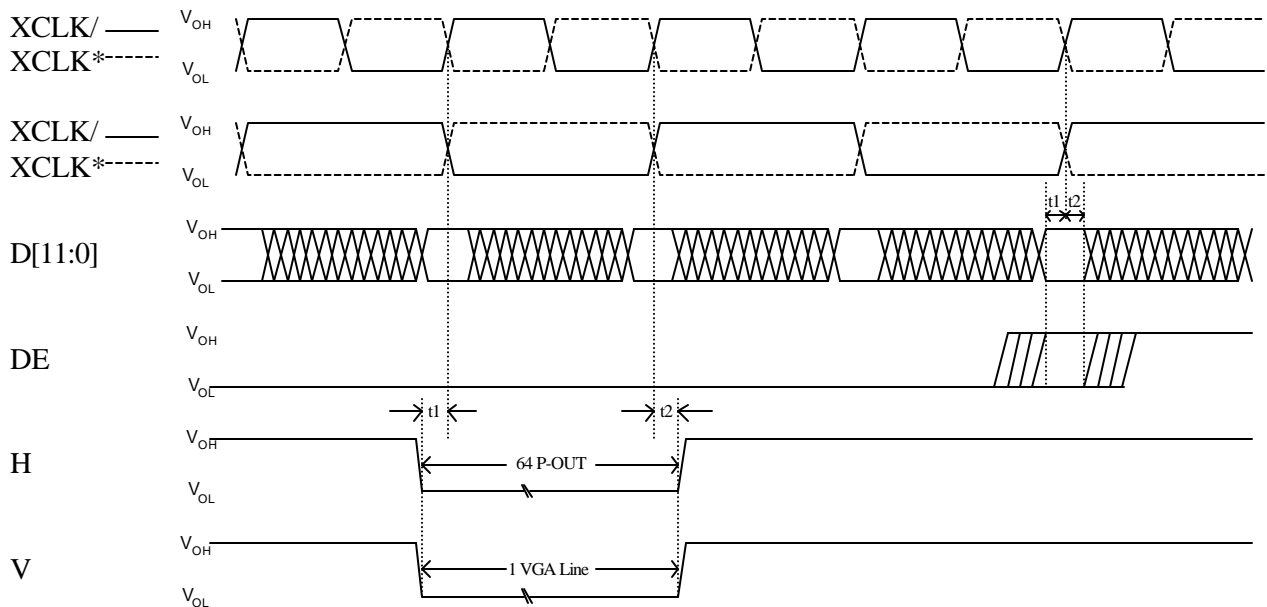
Figure 5: Interface Timing
